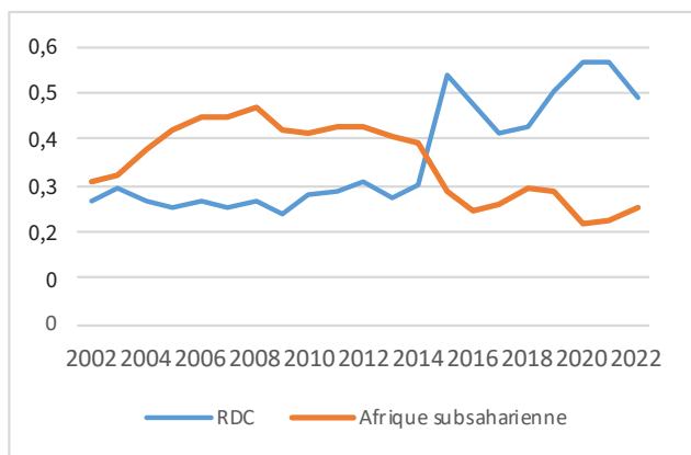
Figure 8a. Indice de concentration : RDC et ASS, 2002-2022
